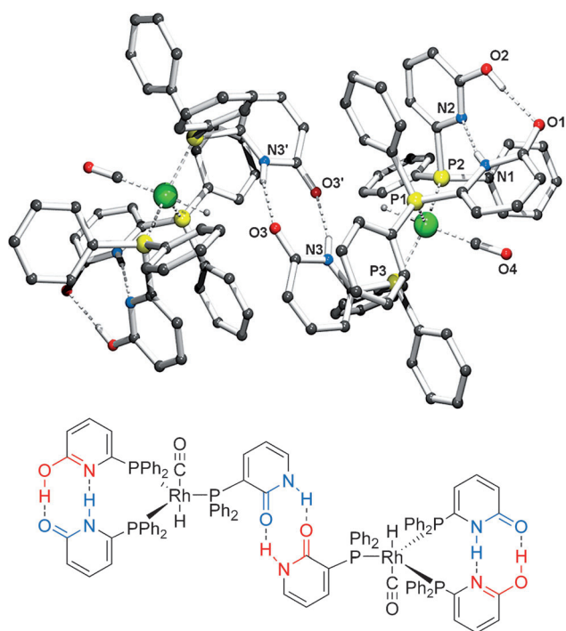
Figure 1. X-ray structure of the [HRh(6-DPPon) 3 (CO)] (4) complex. Selected bond lengths [Å] and angles [°]: N–H...O: 2.880(3), 164(3); O–H...O: 2.657(3), 170(4); N–H...N: 2.892(3), 169(3); P–Rh–P: 115.23(3).
