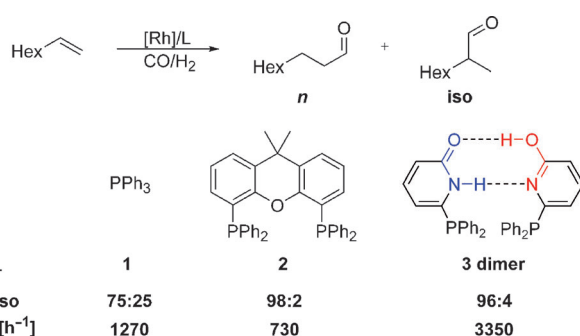
Scheme 1. Selectivity and activity observed in the rhodium-catalyzed hydroformylation of 1-octene with various ligands. Conditions: Rh/L/substrate = 1:20(10):7500, 80 °C, 10 bar, toluene.
